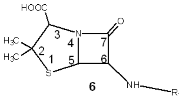
Figure 1: Amoxicillin structure
